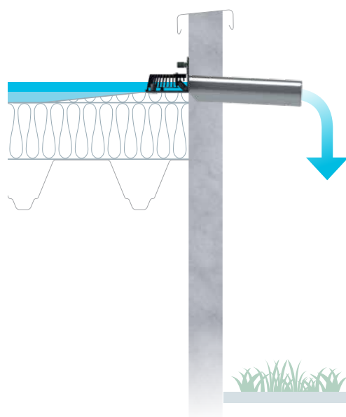
D SitaRondo Above the insulation, led through the parapet as a spout
