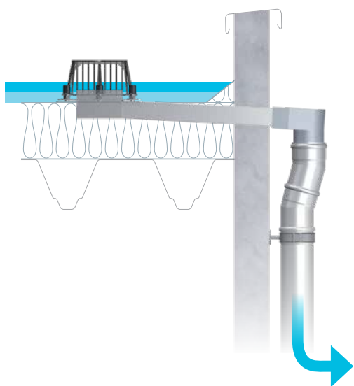
A SitaTurbo with retaining element Passed through the parapet with intervention in the insulation
