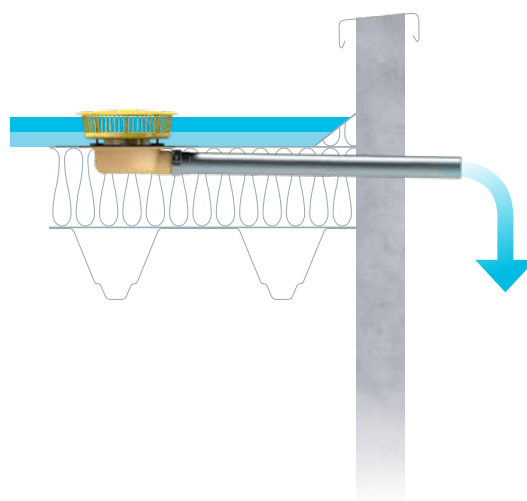
B SitaIndra with retaining element Routed through the parapet with intrusion into the insulation
