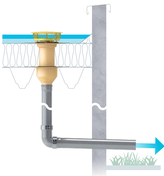
C SitaStandard with SitaPipe stainless steel pipe system Guided through the facade
